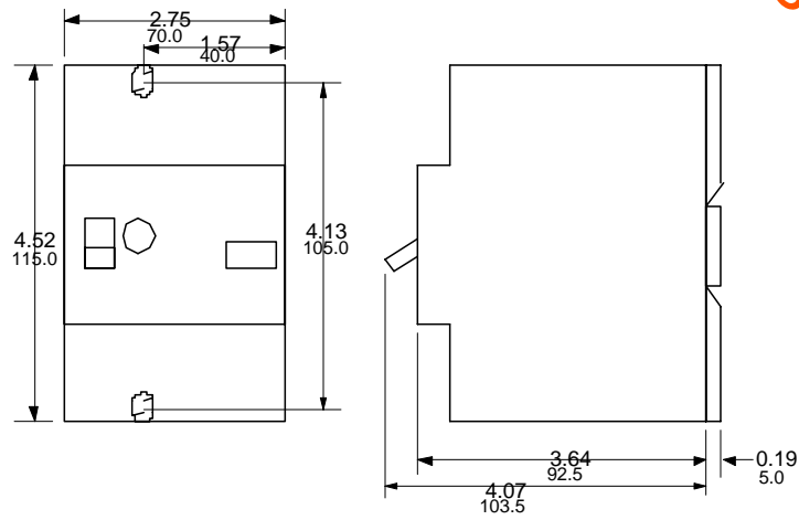
M63TM MANUAL MOTOR STARTER
