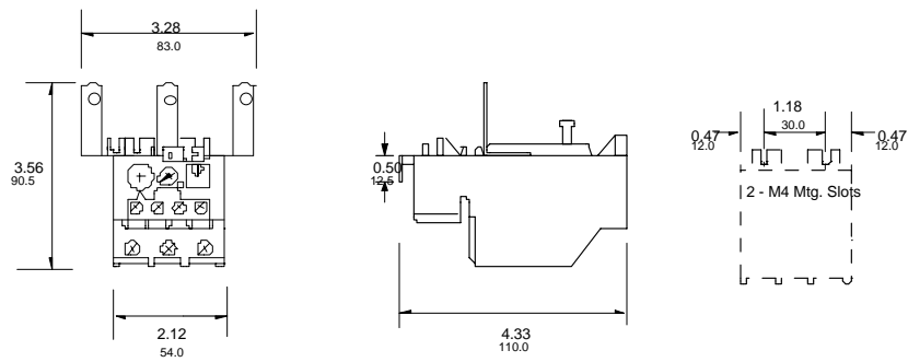
ABB Control Inc. 7/ 7/ 95 T 80 OVERLOAD RELAY
