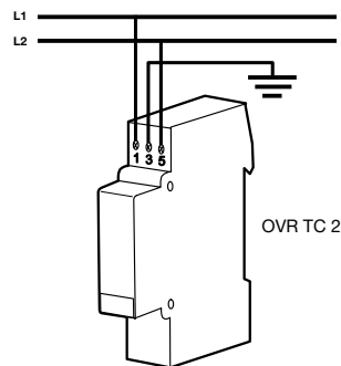
OVR TC 200 V in parallel
