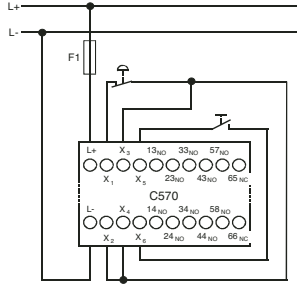
EMERGENCY-STOP circuit
