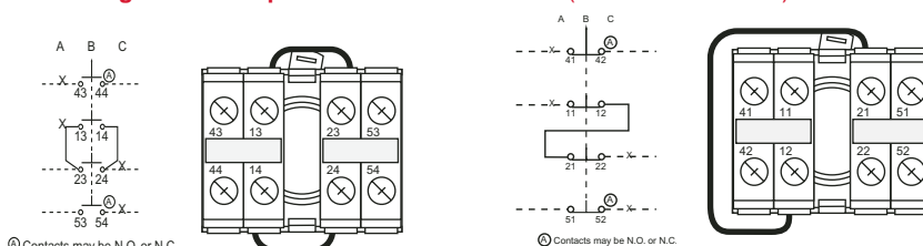
Fig. 1 – Center position connection detail (CBK-TM & CBK-TS)
