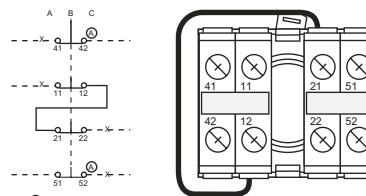
Fig. 1 – Center position connection detail
