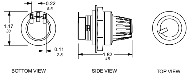
Potentiometer – NEMA 4X without terminal block
