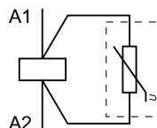
Varistor (only)
