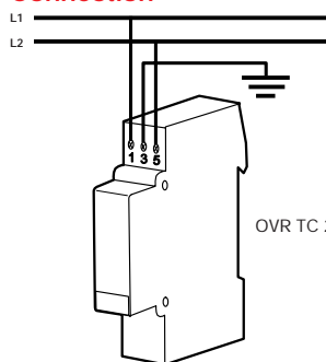
OVR TC 200 V in parallel
