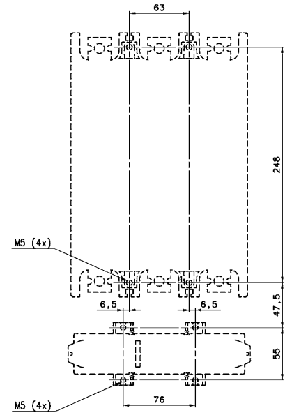
Drilling plan
