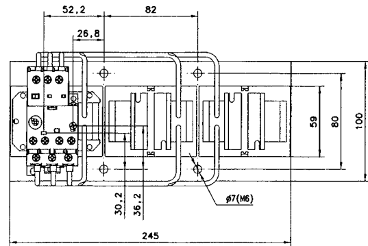
Drilling plan
