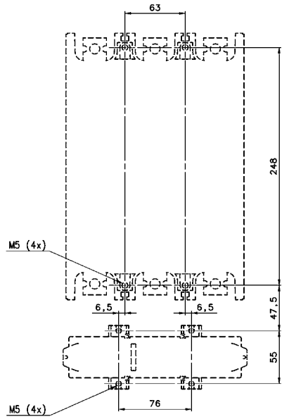
Drilling plan
