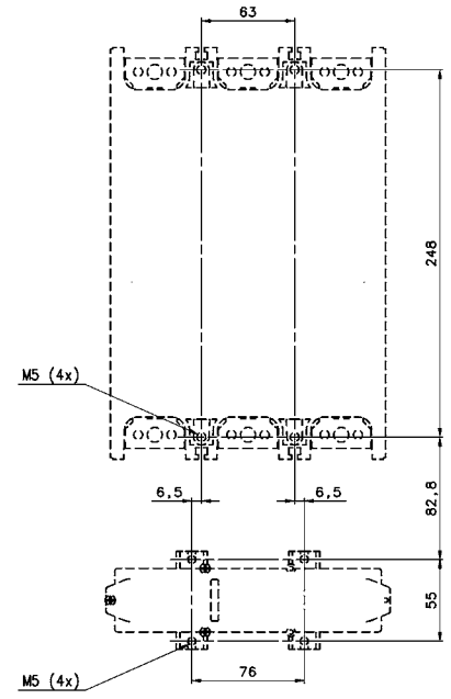
Drilling plan
